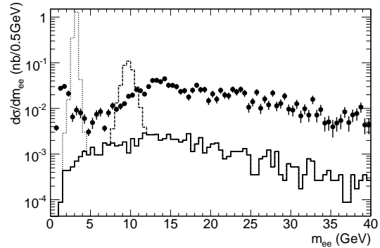
Figure 10.65: Expected differential cross-section for low-mass electron pairs using the 2e5 trigger menu item discussed in section 10.9.3. Shown is the invariant di-electron mass distribution reconstructed using tracks for J/\psi \rightarrow ee decays (dotted histogram), \Upsilon \rightarrow ee decays (dashed histogram) and Drell-Yan production (full histogram). Also shown is the expected background after the offline selection described in the text (full circles).
