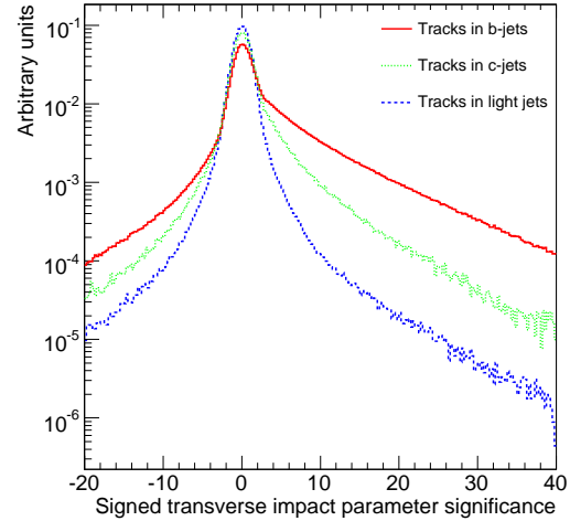
Figure 10.98: Signed transverse impact parameter significance, d_0/\sigma_{d_0} , distribution for b -jets, c -jets and light jets.
