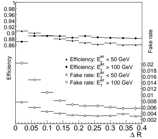
Figure 10.15: Track reconstruction efficiencies and fake rates as a function of the distance \Delta R (defined as \Delta R = \sqrt{\Delta\eta^2 + \Delta\phi^2} ) of the track to the jet axis, using the standard quality cuts and integrated over |\eta| < 2.5 .
