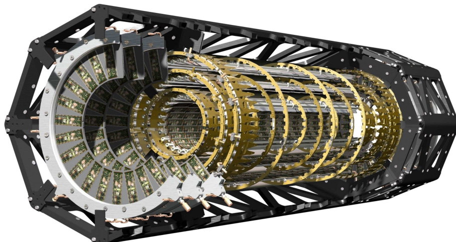
Figure 4.24: A perspective cut-away view of the pixel detector. The view shows individual barrel and end-cap modules, supported with their associated services on staves and disks within an octagonal support frame.
