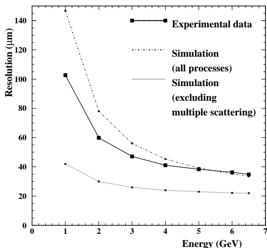
Figure 7.6: The spatial resolution as function of the beam energy compared to GEANT4 simulations with and without the contributions from multiple scattering.
