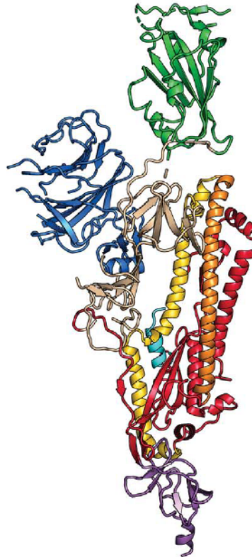
2019-nCoV S RBD up protomer
