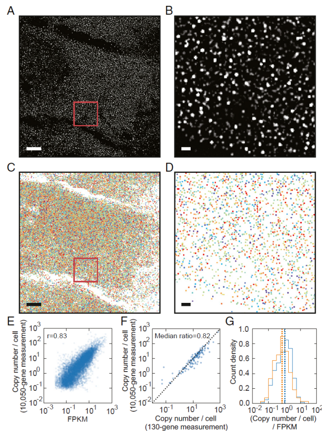
Fig. 1. MERFISH imaging of 10,050 genes in individual U-2 OS cells. (A) A high-pass-filtered, single-z slice, single-bit image of a U-2 OS sample stained with
