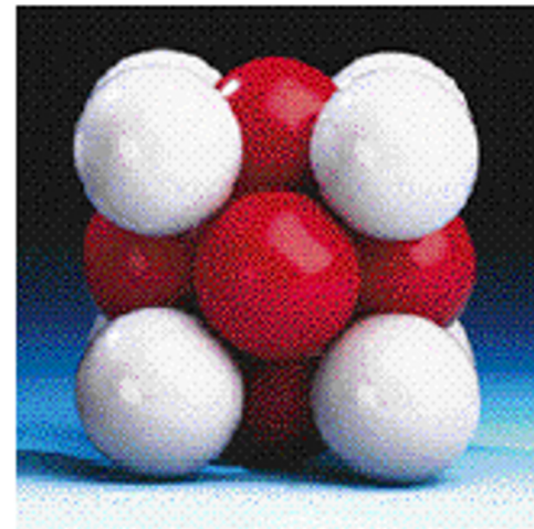
face-centered cubic
