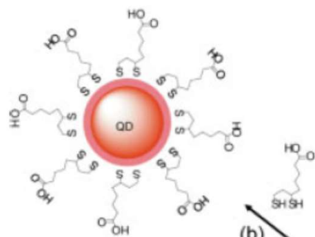
Thiol chelation
