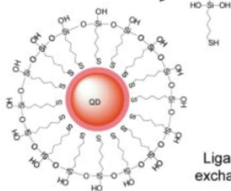
(c) Silanization
