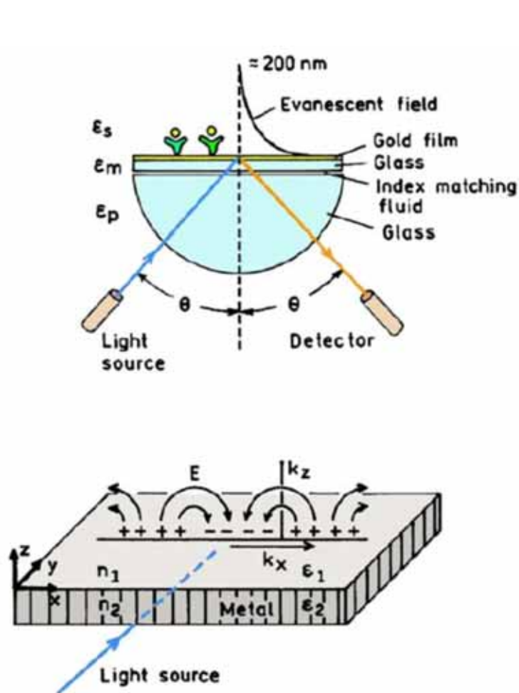
Figure 3. Schematics of an SPR experiment (top) and of the light-induced surface plasmons (bottom).
