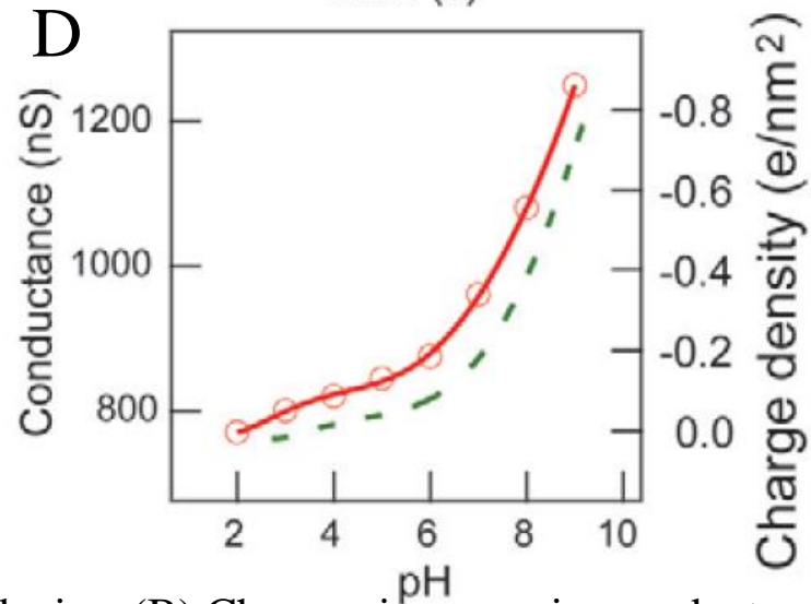
(A) Schematic of an amino-functionalized nanowire device. (B) Changes in nanowire conductance as the pH of solutions delivered to the sensor is varied from 2 to 9; inset is a plot of conductance data versus pH. (C) Schematic of an unmodified nanowire sensor containing silanol groups. (D) Conductance of an unmodified Si nanowire device (red) versus pH.
