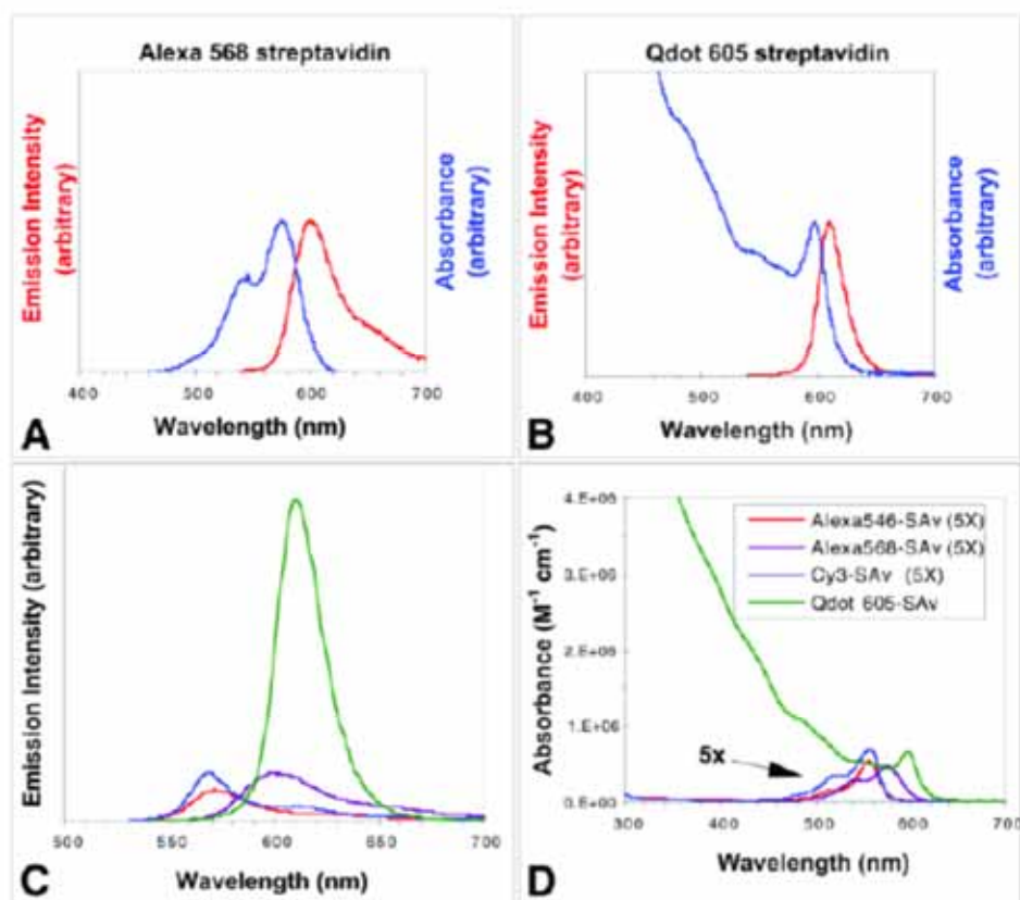
Fig. 1. Comparison of absorbance and emission spectra (normalized) of (A) Alexa® 568 streptavidin conjugate and (B) Qdot® 605 streptavidin conjugate. Note that the quantum dot conjugate can absorb light efficiently far to the blue of the emission. (C) Comparison of emission spectra (nonnormalized) of streptavidin conjugates of Qdot 605 (—), Alexa 546 (—), Alexa 568 (—), and Cy3® (—). The spectra were taken under conditions in which each fluorophore absorbed the same amount of excitation light. The measured quantum yields of the conjugates were 55, 8, 16, and 11%, respectively. (D) Comparison of absorbance spectra (nonnormalized, each 1 \mu M fluorophore) of Qdot 605 streptavidin conjugate (—), Cy3 streptavidin conjugate (—), Alexa 546 streptavidin conjugate (—), and Alexa 568 streptavidin conjugate (—). Note that all dye spectra are enhanced fivefold for clarity. Alexa, Cy3, and Qdot are registered trademarks of Molecular Probes, Amersham Biosciences, and Quantum Dot Corporation, respectively.
